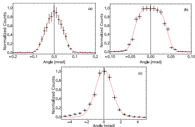
Fig. 2. RC measurements. (a) PWO; (b) BGO; (c) CsI. The dashed red lines are the fitted function to find the mosaicity of the samples.
