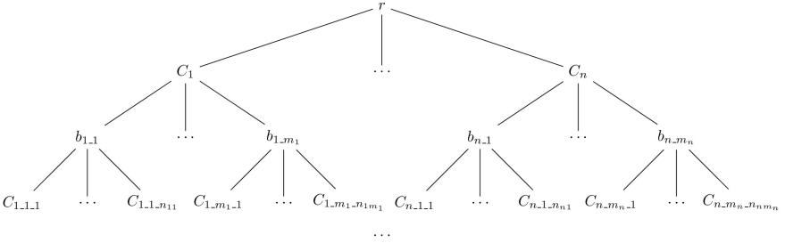
Fig. 4: Generic Hierarchical Probabilistic Logic Program
