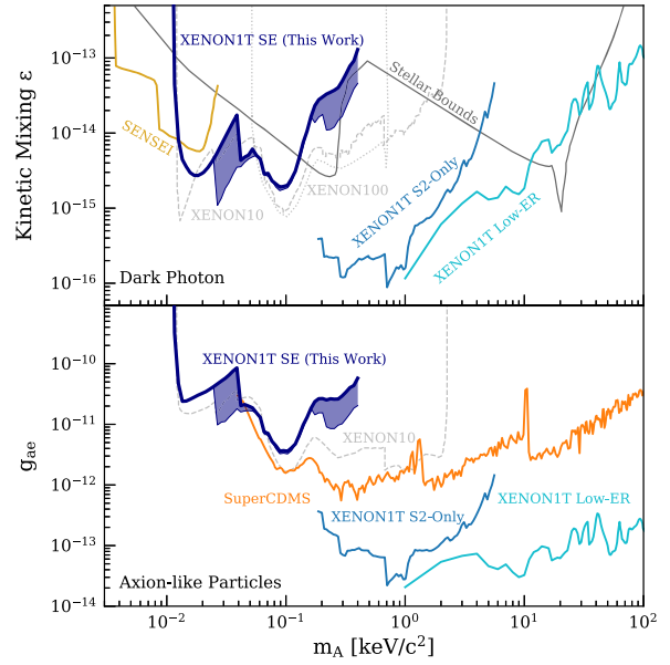
FIG. 15. The 90% confidence level upper limits on bosonic DM (dark blue) via dark photons (top) and ALPs (bottom), as a function of DM mass m_A . The blue shaded band indicates the systematic uncertainty induced by the unknown differential ionization rate of the various electron shells in xenon. For comparison, we show experimental results (solid) from XENON1T S2 only [10] (light blue), XENON1T low ER [46] (cyan), SENSEI [52] (gold), and SuperCDMS [57] (orange), alongside limits calculated (gray) in Ref. [38] using data from XENON10 [11] (dashed) and XENON100 [15] (dotted). Also shown are astrophysical constraints [58] (dark gray).
