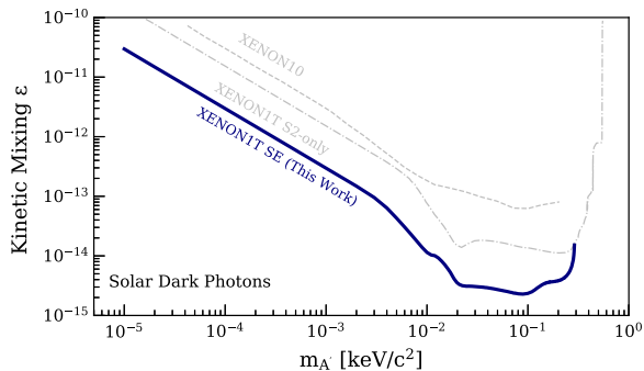
FIG. 16. The 90% confidence level upper limits on bosonic DM via solar dark photons (dark blue), as function of DM mass m_A . For comparison, we show limits calculated (gray) in Ref. [59] using data from XENON10 [11] (dashed) and Ref. [60] using data from XENON1T S2-only [10] (dot dashed).
