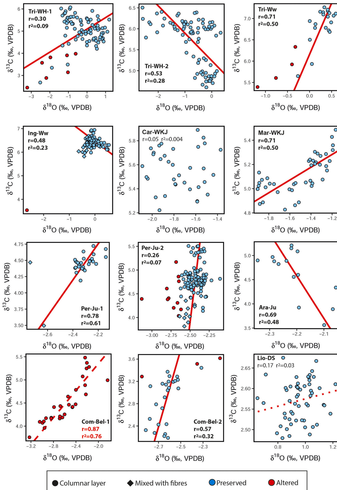
Fig. 5. Cross plots of shell \delta^{18}\text{O} and \delta^{13}\text{C} values of the samples. Circles and diamonds represent samples from the columnar layer and those contaminated by sampling of fibrous layer; Cyan color represents samples deemed to be preserved, and red are altered samples. The regression line, r , and r^2 are calculated for preserved samples of the columnar layer; in the specimen Com-Bel-1 the calculation refers to altered samples. (For interpretation of the references to color in this figure legend, the reader is referred to the web version of this article.)
