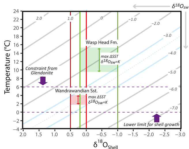
Fig. 12. Estimated of maximum \Delta\text{SST} for the Wasp Head Formation (green) and Wandrawandian siltstone (red). Lines and shaded areas refer to the estimated for minima and maxima \delta^{18}\text{O} values of the overlapping ranges observed from shells of similar ages for the anterior part of the columnar layer. The maximum \Delta\text{SST} are estimated assuming constant \delta^{18}\text{O}_{\text{sw}} values equal to -2.0 ‰ for Wasp Head Formation (Frank et al., 2015) and \sim -3.5 ‰ for Wandrawandian Siltstone. (For interpretation of the references to color in this figure legend, the reader is referred to the web version of this article.)
