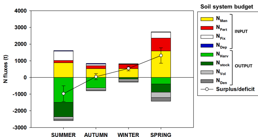
Fig. 2. Components of the Soil System Budget (SSB) of nitrogen (N) for the study area within the Mincio River watershed for all seasons. N_{Man} = N in livestock manure applied to agricultural soils; N_{Fert} = N in synthetic fertilizer applied to agricultural soils; N_{Fix} = agricultural N_2 fixation associated with N fixing crops; N_{Dep} = atmospheric N deposition on agricultural land; N_{Harv} = N exported from agricultural soils with crop harvest; N_{stock} = organic N in crop's standing stock; N_{Vol} = NH_3 volatilization in agricultural soils; N_{Den} = denitrification in agricultural soils. White dots represent seasonal N budgets ( \Sigma INPUTS - \Sigma OUTPUTS); positive values suggest surplus whereas negative values suggest deficit.
