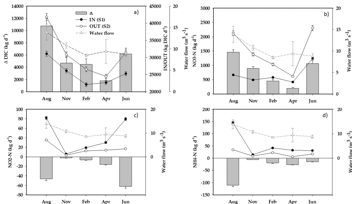
Fig. 5. Daily loads of inorganic carbon (DIC; a), nitric nitrogen (NO3-N; b), nitrous nitrogen (NO2-N; c), and ammonium nitrogen (NH4-N; d) transported at the extremes of the studied river reach and their differences ( \Delta = S2-S1 ) in the period August 2016 to June 2017. Water flow is also reported. Mean values are given, with error bars corresponding to \pm 1 standard deviation.
