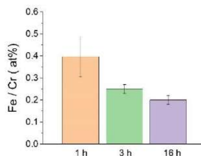
Figure SEQ Figure (* ARABIC 1): Fe/Cr atomic percentage ratio on steel exposed 1 h, 3 h and 16 h to D solution.
