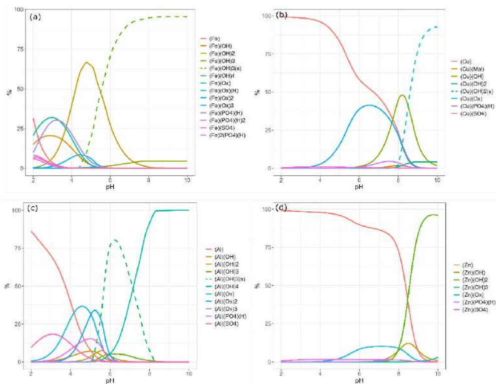
Figure 1: Species distribution diagrams of (a) Fe 3+ , (b) Cu 2+ , (c) Al 3+ , and (d) Zn 2+ occurring in the soluble fraction of Arctic PM 10 collected in 2012 as a function of pH.
