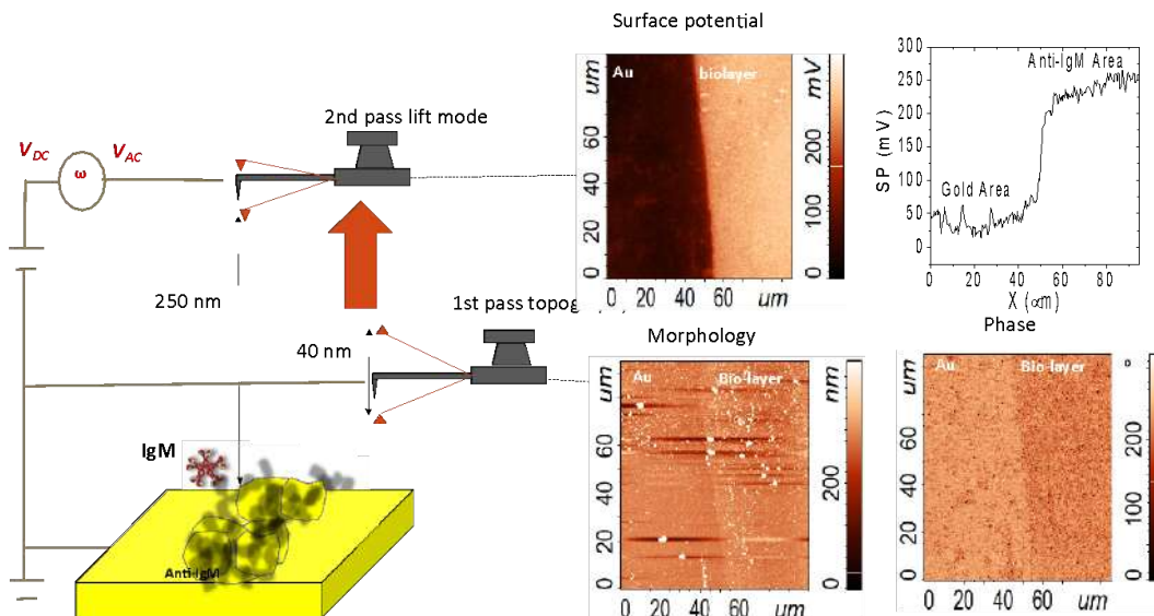
Figure 1: Kelvin Probe Force Microscopy quantitative analysis for antigen/antibody recognition process.
