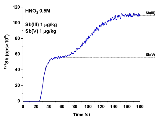
Figure 1: Frontal chromatogram of a 1 μg/kg Sb(V) and Sb(III) solution obtained under optimized conditions.
