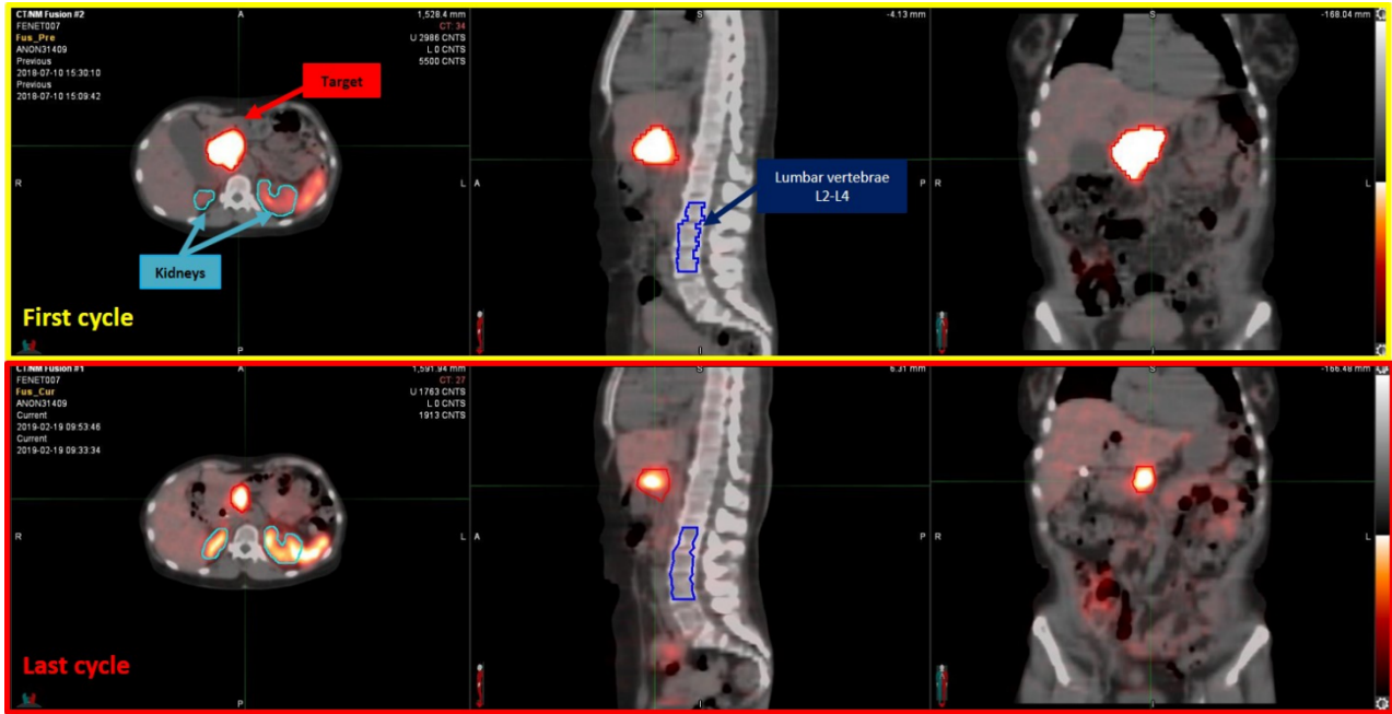
Figure 2 Example of segmentation of the OARs and targets at first and last cycles via MIM® Maestro workstation using SPECT/CT data and segmentation propagation for kidneys and BM.
