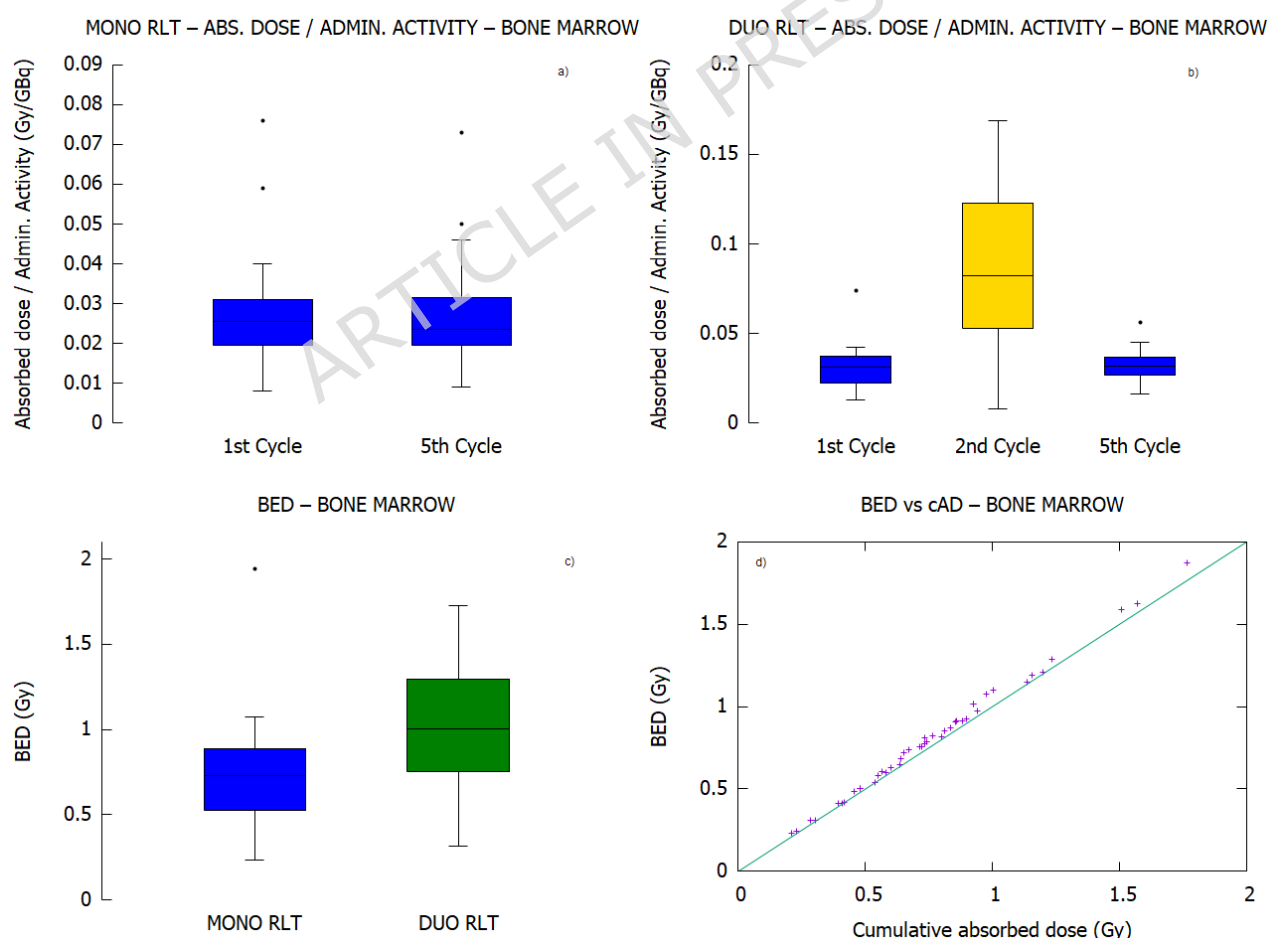
Figure 4 Absorbed doses per administered activities for BM for MONO (a) and DUO (b) RLT. BED for MONO and DUO RLT (c) and correlation between BED and AD (d) for BM.
