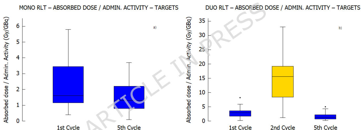
Figure 5 Absorbed doses per administered activities for targets for MONO a) and DUO b) RLT. Results are shown per cycle: 1 st and 5 th for MONO, 1 st , 2 nd and 5 th for DUO RLT.
