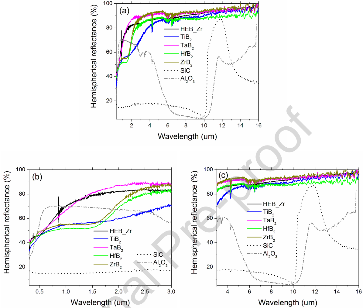
Figure 5: Comparison of the hemispherical reflectance spectra of HEB_Zr and monolithic TiB 2 , TaB 2 , HfB 2 and ZrB 2 (from [18,20,22]). Spectra of SiC and Al 2 O 3 are also included for reference (from [42]). (a) Full spectral range and details of (b) 0.3-3 μm range and (c) 3-16 μm range.
