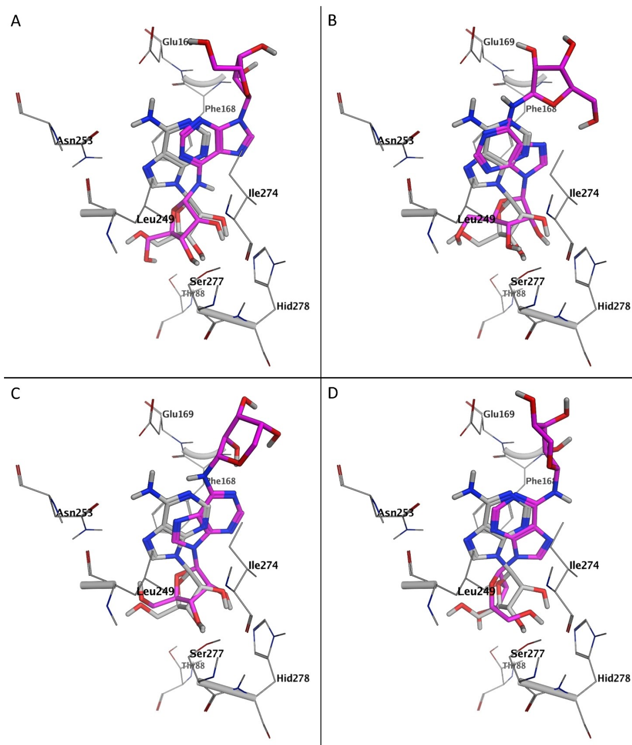
Figure 6. This panel reports the superposition of the best docking pose within the orthosteric binding site of the A2 A adenosine receptor for each of the four solution species of N6-(D-ribose-1-yl)-adenosine (magenta) and the crystal pose of adenosine (grey). A) \alpha -FUR. B) \beta -FUR. C) \alpha -PYR. D) \beta -PYR.
