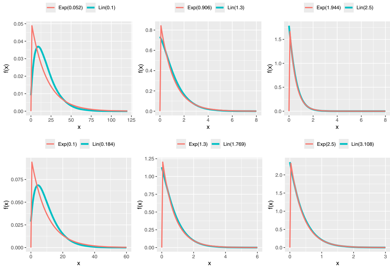
Fig. 3 Probability density function f(x) of Lindley (Lin) and exponential (Exp) distributions for different parameters
