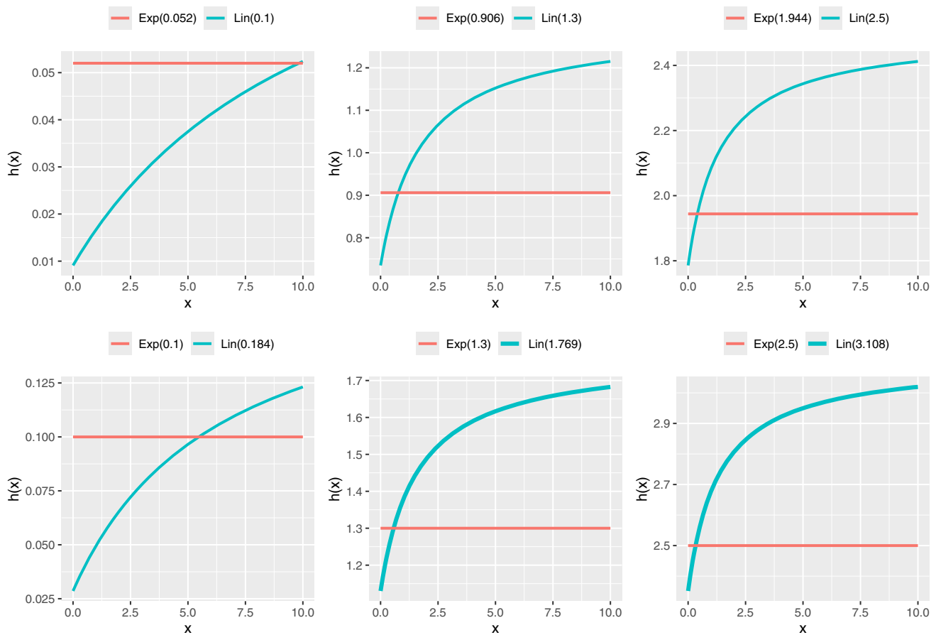
Fig. 5 Hazard rate function h(x) of Lindley (Lin) and exponential (Exp) distributions for different parameters
