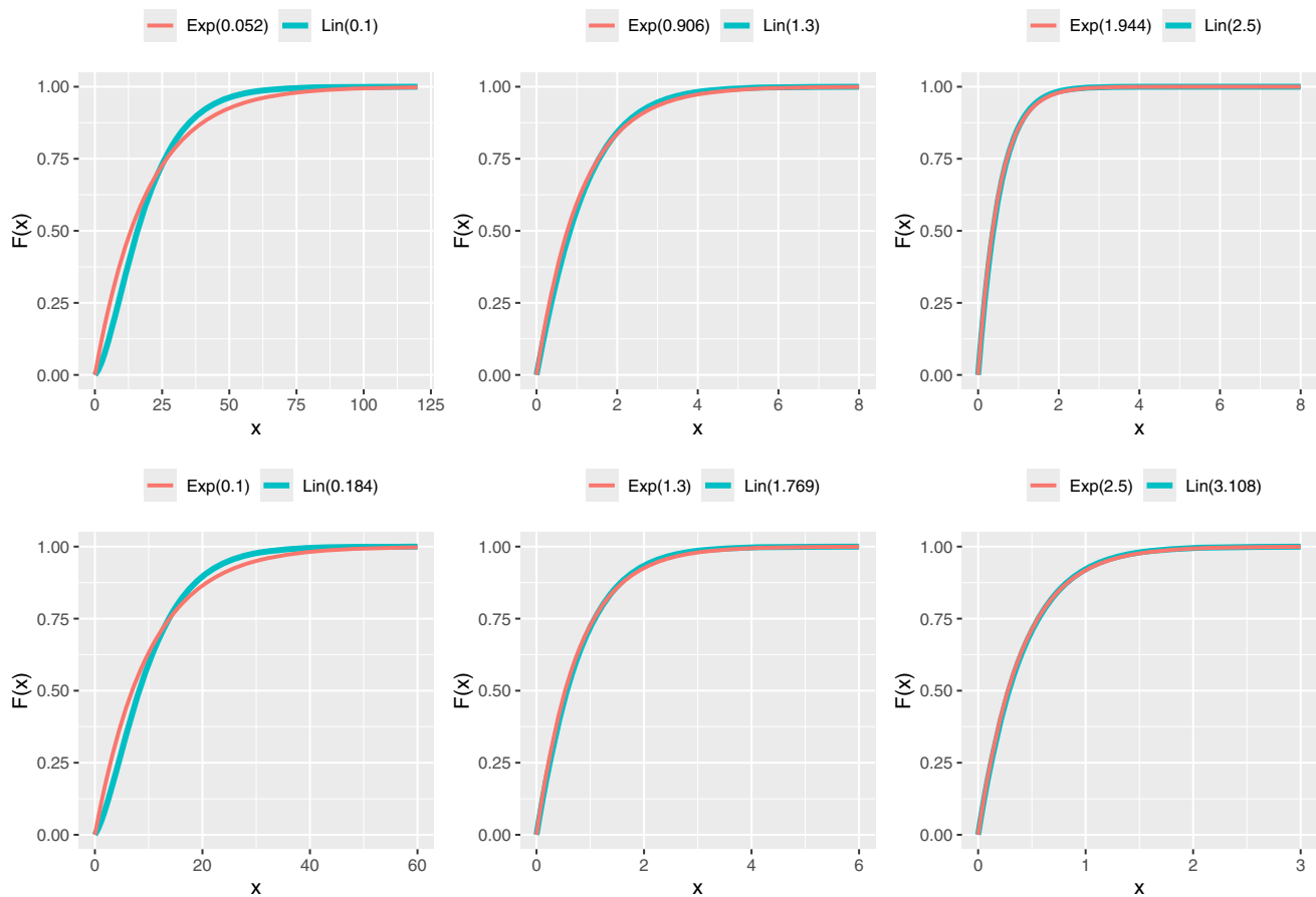
Fig. 4 Cumulative density function F(x) of Lindley (Lin) and exponential (Exp) distributions for different parameters
