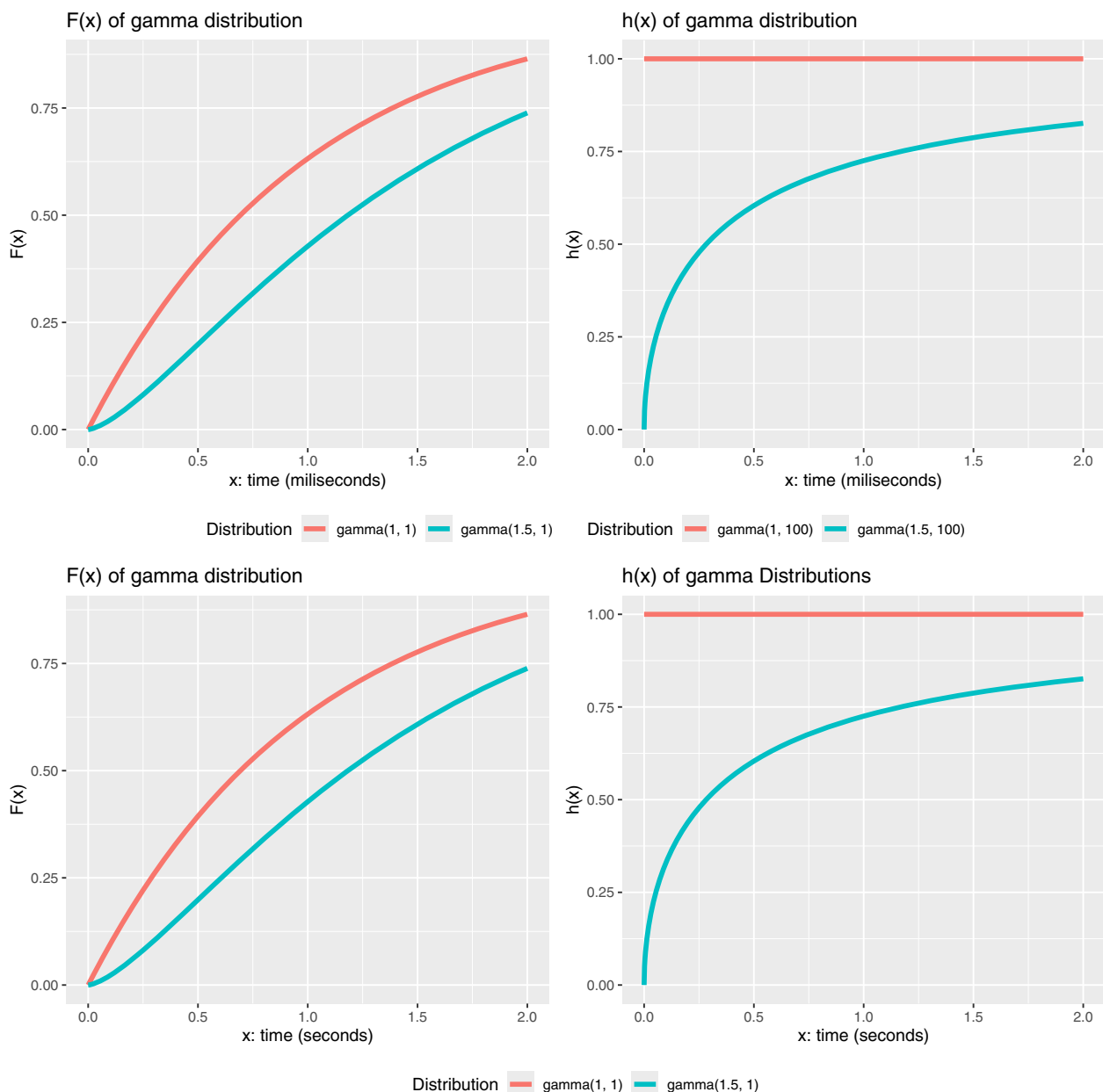
Fig. 2 Distributions modeled with gamma distributions. The distributions have positive skewness ( first column ) but different hazard rate functions ( second column ). The same data are presented in two analogous metrics
