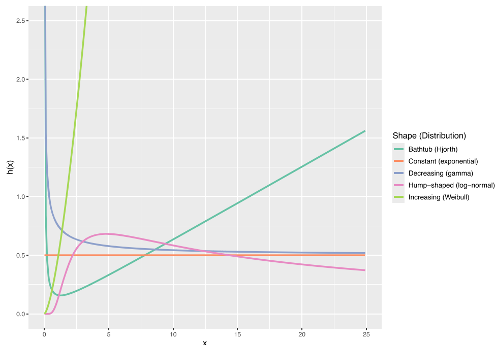
Fig. 1 Illustration of hazard rate function h(x) shapes corresponding to different probability distributions: Hjorth (Bathtub), exponential (Constant), gamma (Decreasing), log-normal (Hump-shaped), and Weibull (Increasing)
