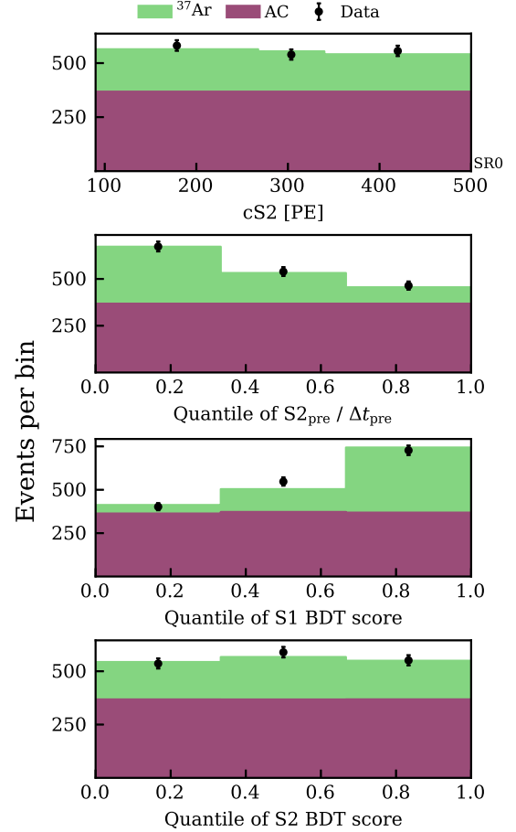
FIG. 6. Distributions of the best-fit AC background, ^{37}\text{Ar} L shell EC signal, and the observed data in the ^8\text{B} CE \nu NS analysis dimensions. The observed number of events with Poisson uncertainties in each bin is shown in black. The ^{37}\text{Ar} signal (AC background) is shown by the green (purple) histogram.
