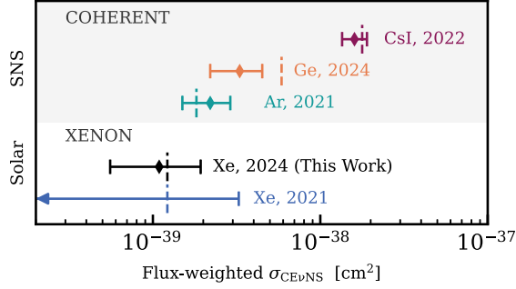
FIG. 4. Measurements of the flux-weighted CE \nu NS cross section \sigma_{\text{CE}\nu\text{NS}} . The measurement using Xe nuclei solar ^8\text{B} neutrinos from this work is shown in black. The 90% CL upper limit from XENON1T [7] is shown in blue. The measurements with neutrinos from the SNS by the COHERENT Collaboration using CsI [44] (red), Ar [5] (green), and Ge [45] (orange) nuclei are also shown. For comparison, the SM predictions are shown by vertical dashed lines.
