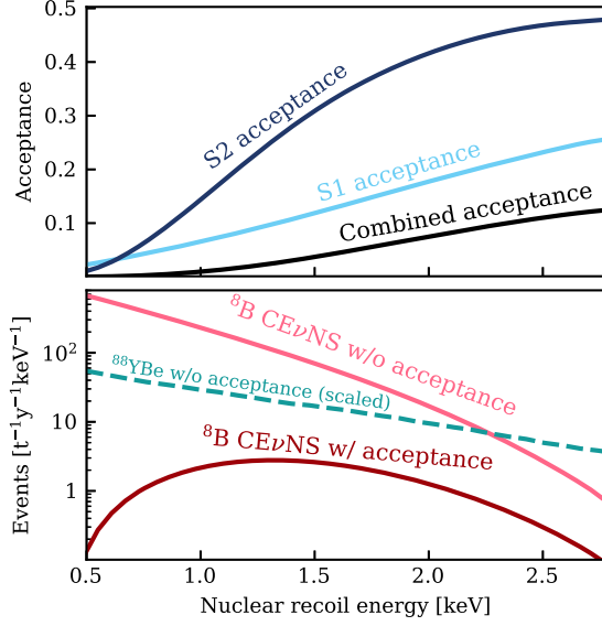
FIG. 1. Acceptance for detecting low-energy NRs in XENONnT (top) and ^8\text{B} CE \nu NS energy spectrum (bottom). The light (dark) blue curve denotes the acceptance of detecting S1 ( S2 ) signals, and the black curve represents the combined acceptance. The expected CE \nu NS signal spectrum induced by solar ^8\text{B} neutrinos in XENONnT with (without) acceptance loss is shown by the dark (light) red line. The green line shows a scaled spectrum of all energy depositions from ^{88}\text{YBe} calibration.
