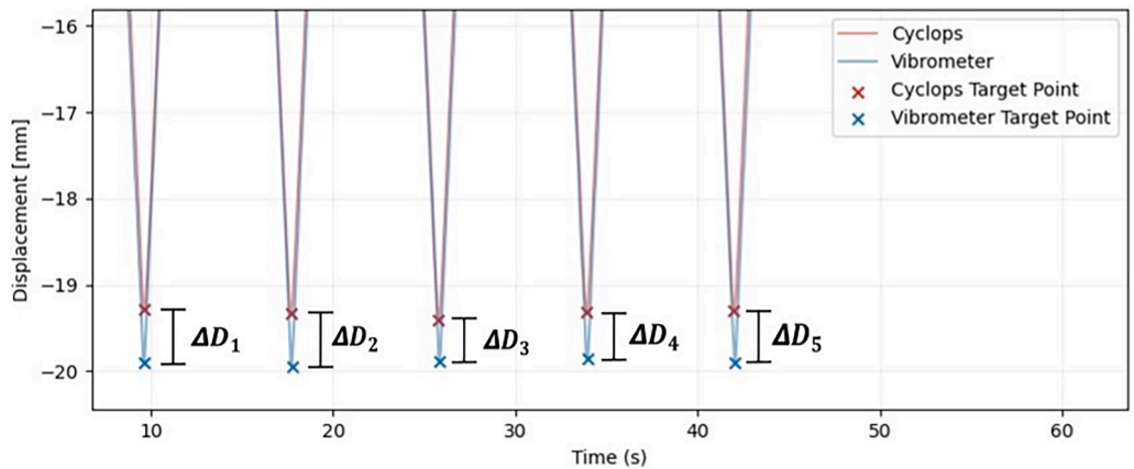
Fig. 5. Difference \Delta D evaluated on the maximum displacement between the signals obtained with the JTS and with the reference LDV.
