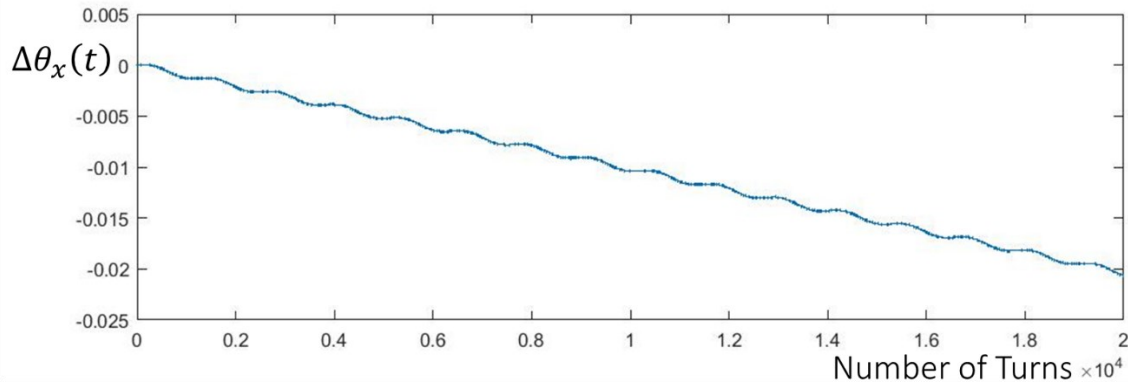
Figure 49: A plot showing the spin tune spread of the polarisation vector measured simultaneously with the experiment in Figure 46.
