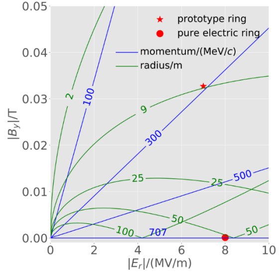
Figure 36: Bending radius (green curves) and particle momentum (blue lines) contours plotted as a function of electric and magnetic fields. The red star plots the configuration of the prototype ring (currently investigated in this thesis) and the red circle plots that of the all-electric ring (described in section 3.2.3) [83]
