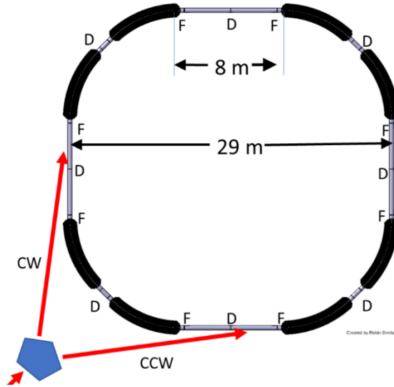
Figure 25: Basic layout of the prototype ring, consisting of eight dual superimposed electric and magnetic bends and two families of quadrupoles ( F , focusing; D , defocusing), with an optional skew quadrupole family at the midpoints. [8]
