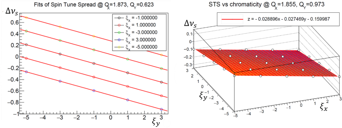
Figure 52: Plots showing the variation of spin tune error with chromaticity. The left plot shows 1D scans varying \xi_y at different fixed values of \xi_x . The right plot shows a 2D scan of a mesh of points that were accurately fit with a plane, whose equation is expressed on top.
