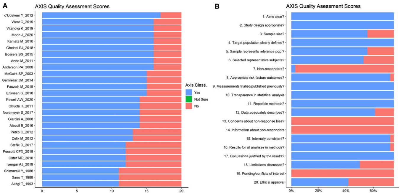
Figure 2: Summary of quality assessment of reports using AXIS. (A) Selected studies sorted by overall quality and (B) rate of fulfilment of each quality item of AXIS across selected papers. Blue colour indicates AXIS criteria fully satisfied; red colour indicates AXIS criteria not satisfied. AXIS: Appraisal tool for Cross-Sectional Studies.
