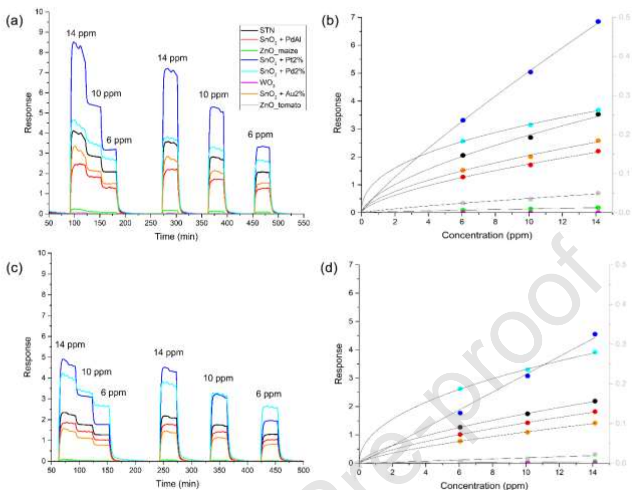
Figure 5. Dynamic response and calibration curve of sensors tested with 14, 10 and 6 ppm of ethylene at 33 %RH a) and b), at 52 %RH c) and d).
