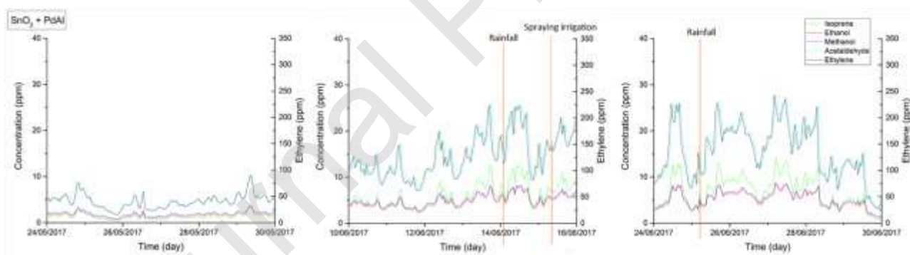
Figure 9. On-field maize gaseous emission concentration detected by SnO 2 + PdAl sensor,
