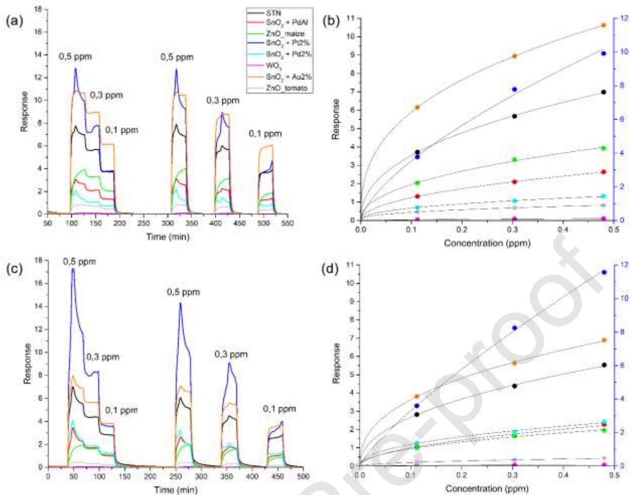
Figure 6. Dynamic response and calibration curve of sensors tested with 0.5, 0.3 and 0.1 ppm of isoprene at 33 %RH a) and b), at 52 %RH c) and d).
