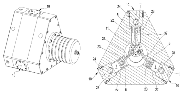
Figure 2 StarEngine piston expander prototype [26]
