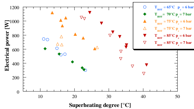
Figure 8 – Expander electrical power vs. superheating degree, for different T_{hot} and p_c values
