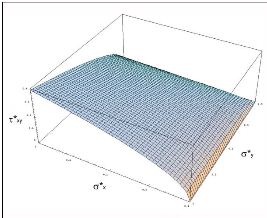
Figure 4.9 Rankine damage threshold surface in the fictitious space.
