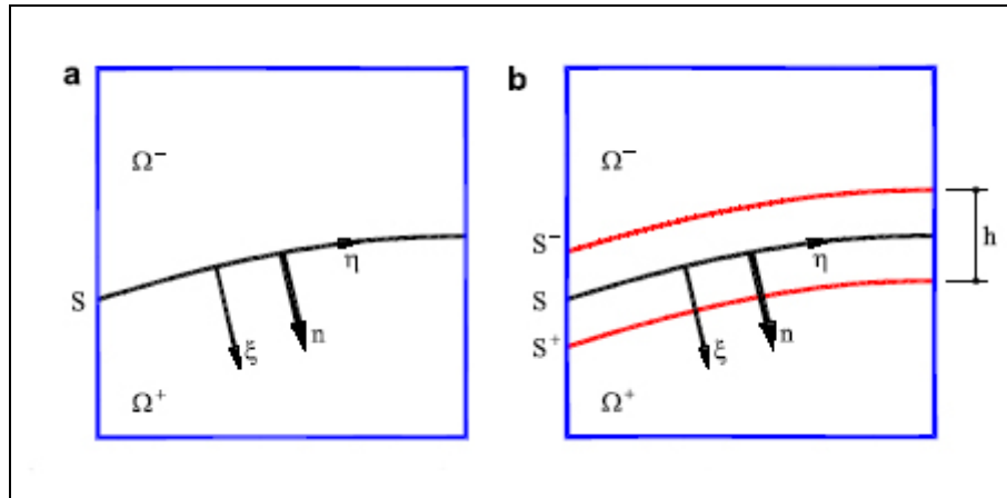
Figure 5.1 Crack modelling at continuum level: discrete approach (a) and smeared approach (b).
