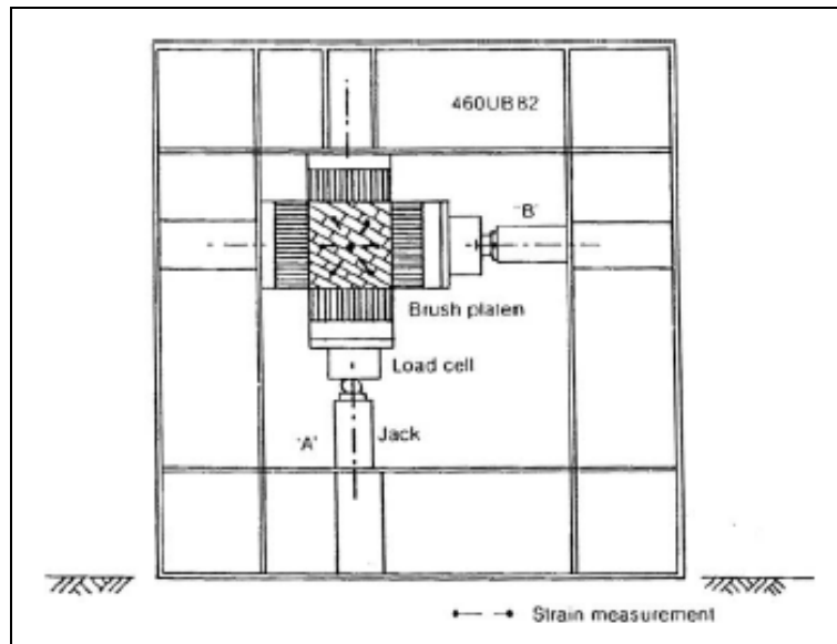
Figure 4.18 Page test setup.
