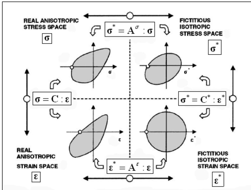
Figure 3.3 Relationship between the fictitious isotropic and the real anisotropic spaces (from Oller et al. , 2003).
