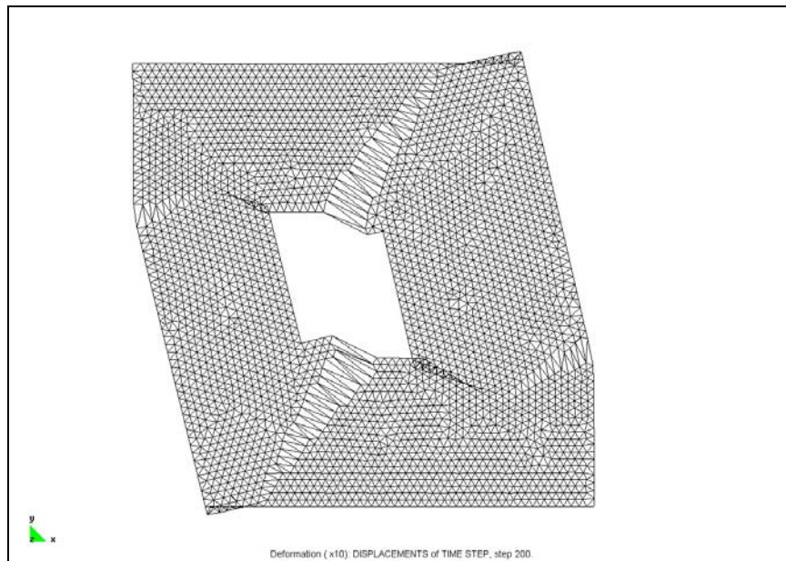
Figure 5.20 Computed deformed mesh (x10).
