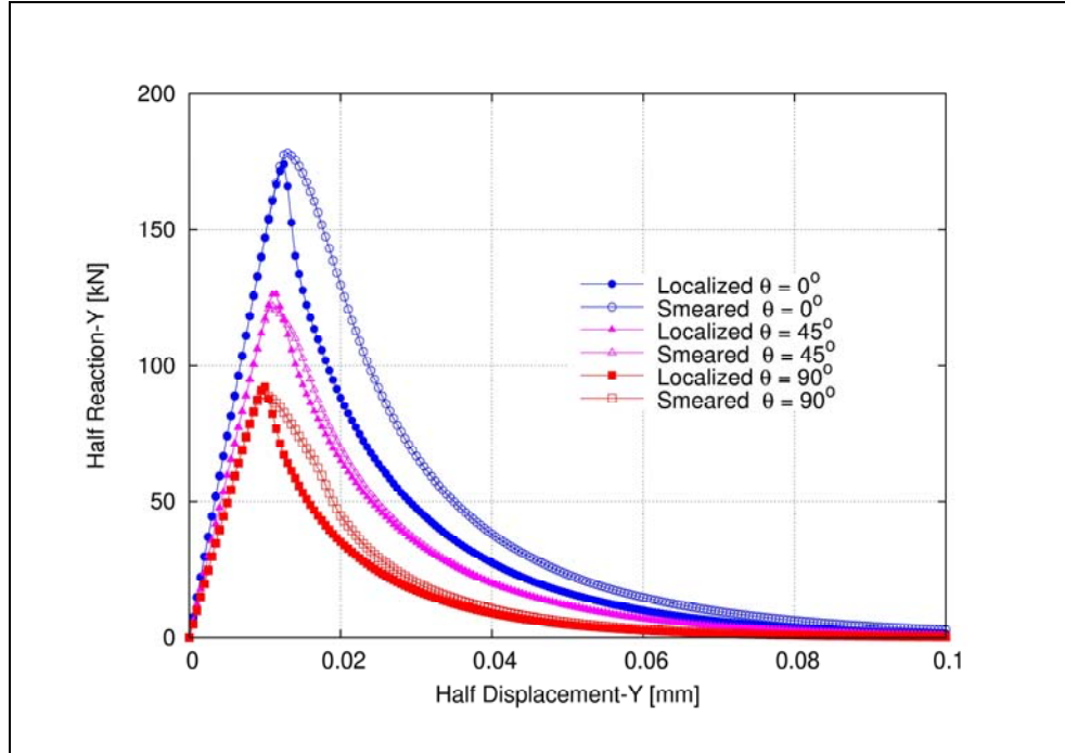
Figure 5.15 Load versus displacement for holed strips with different orthotropy angles. Comparison between localized and smeared damage models.
