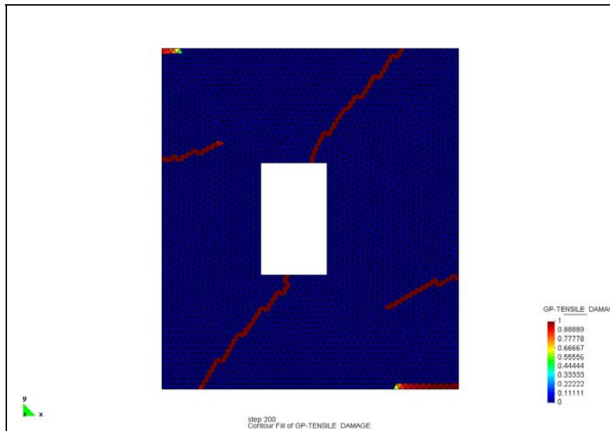
Figure 5.21 Tensile localized damage contour.
