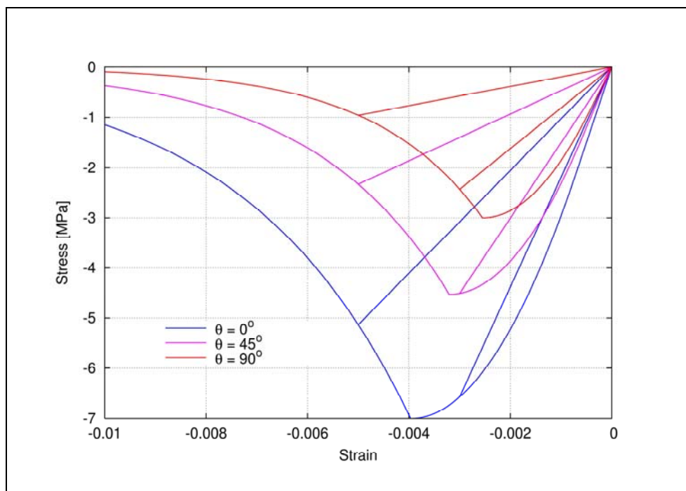
Figure 3.11 Uniaxial compression and unloading to origin.
