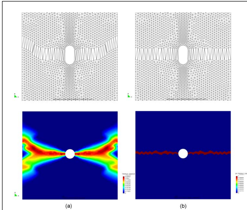
Figure 5.14 Deformed mesh (x100) and tensile damage contour: smeared damage model (a) and localized damage model (b).
