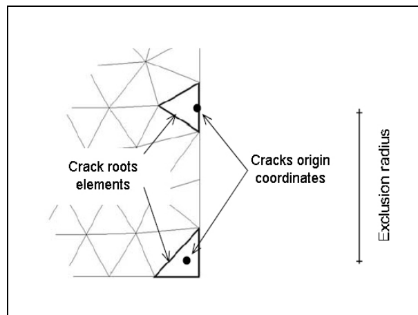
Figure 5.7 Location of cracks origin coordinates.
