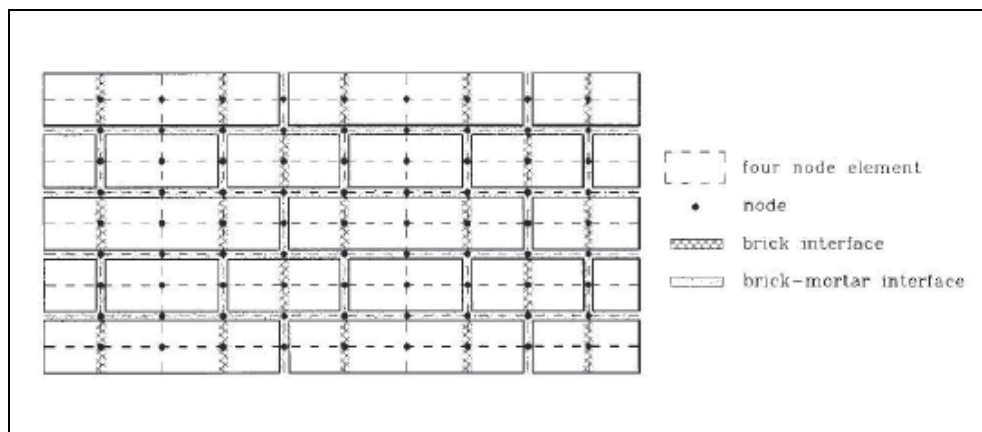
Figure 1.6 Micro-modelling of masonry, from Gambarotta and Lagomarsino (1997a).
