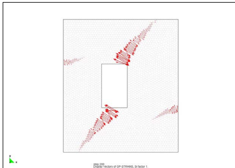
Figure 5.22 Vectors of maximum principal strain.
