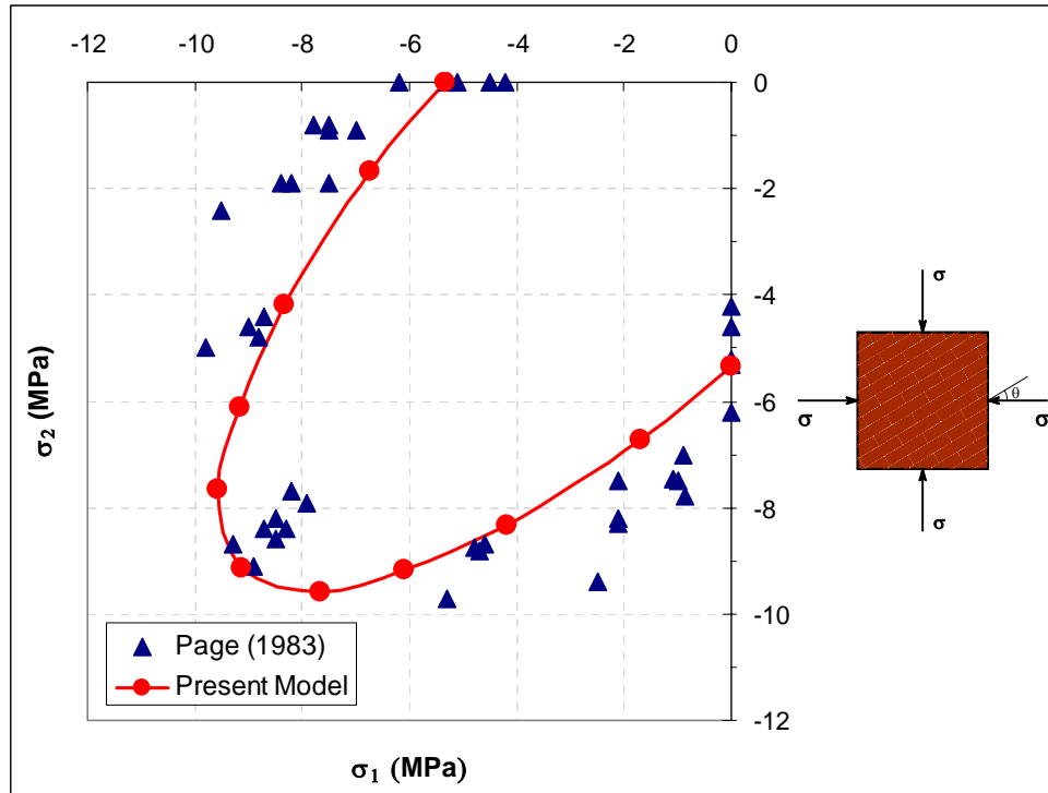
Figure 3.24 Failure envelope for biaxial compression –compression ( \theta = 45^\circ ).
