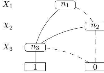
Figure 2: BDD for function (24).
