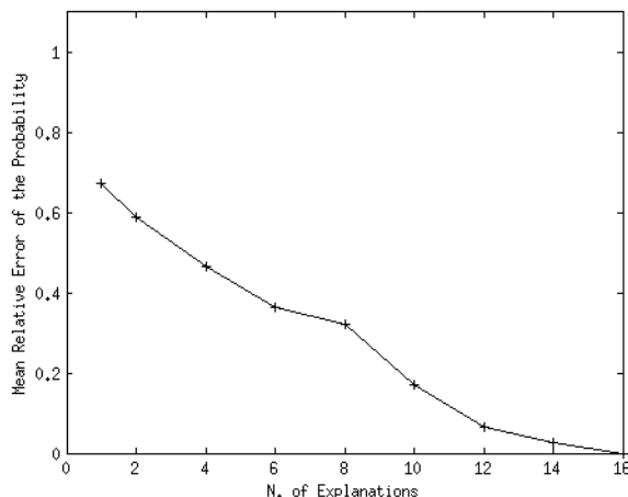
Figure 10: Mean relative error of the probability of queries as a function of the limit on the number of explanation varies.
