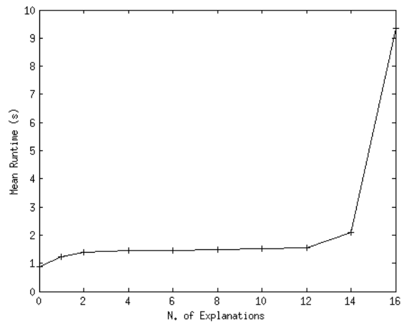
Figure 11: Execution time as the limit on the number of explanations to the queries varies.
