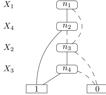
Figure 4: BDD for Example 6.
